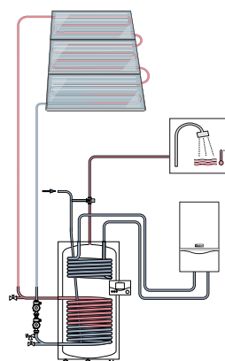
auroSTEP plus 350 + ecoTEC plus VC of ecoTEC exclusiv VC
